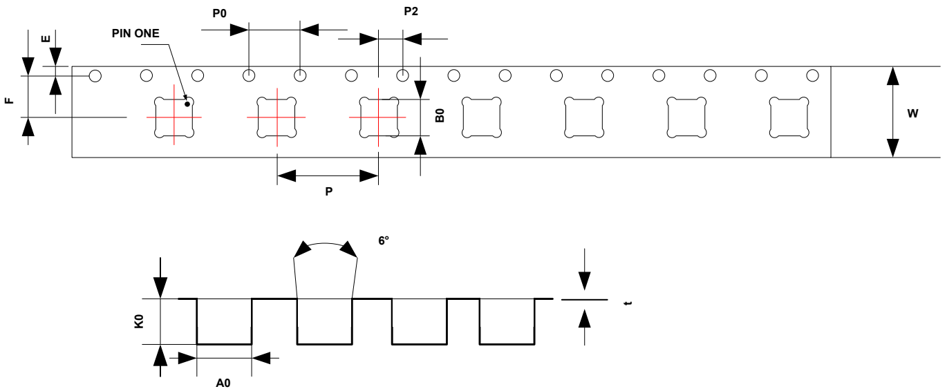
Figure 45 Tape Dimension
