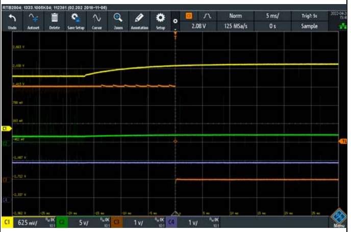
Figure 24 OVP for DCM CH1: VOUT CH2: VIN CH3: PG CH4: IOUT
