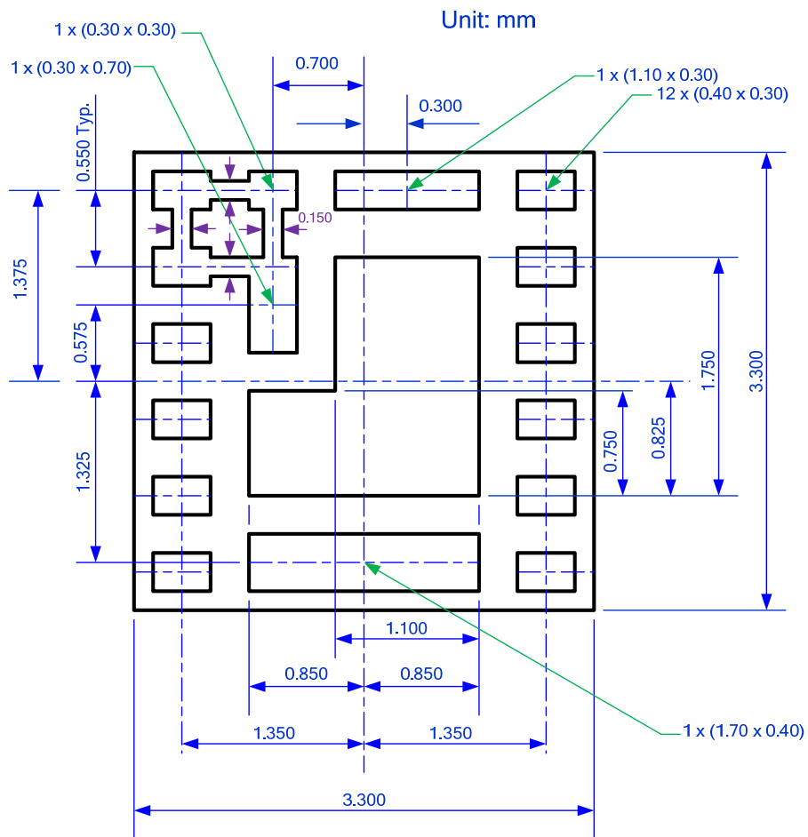
Figure 41 Bottom View
