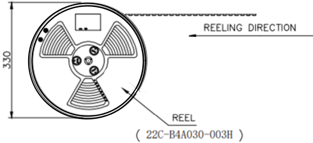
Figure 44 Reel Dimension
