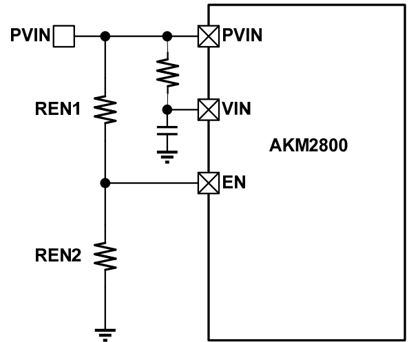
Figure 27. Single supply configuration: internal LDO regulator, adjustable PVIN UVLO
