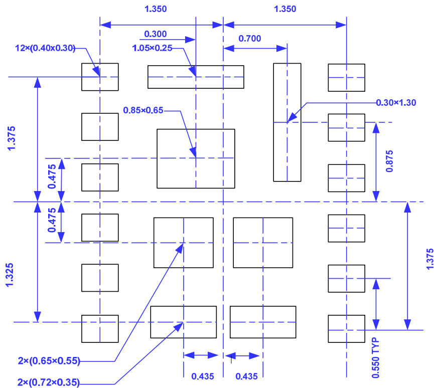
Figure 43 Solder stencil
