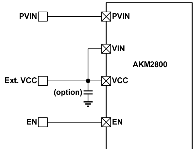
Figure 28 Using external bias voltage
