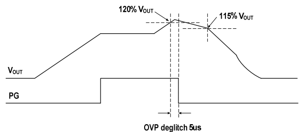
Figure 34. OVP latch-off mode behavior
